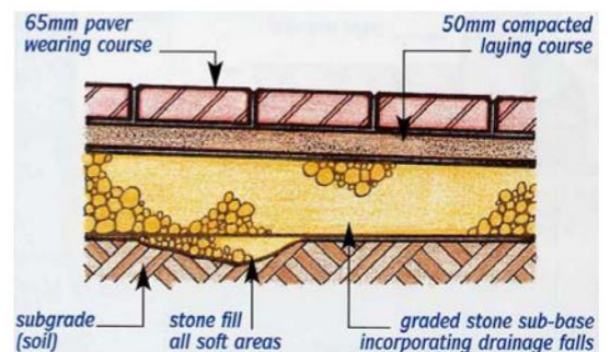
Incorporate the drainage fall in the sub-base
